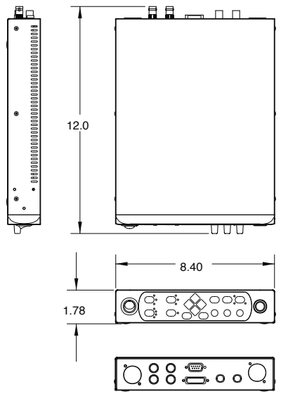
Controller
