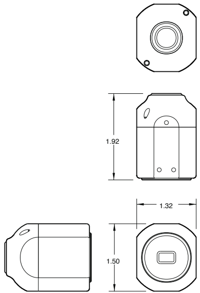
Camera Head
